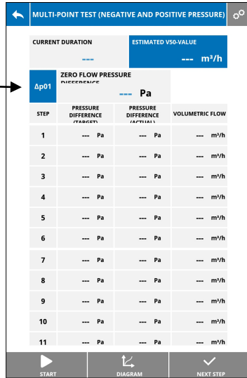
Fig. 55: Multi Point Test view, before the measurement of the zero-flow pressure difference
